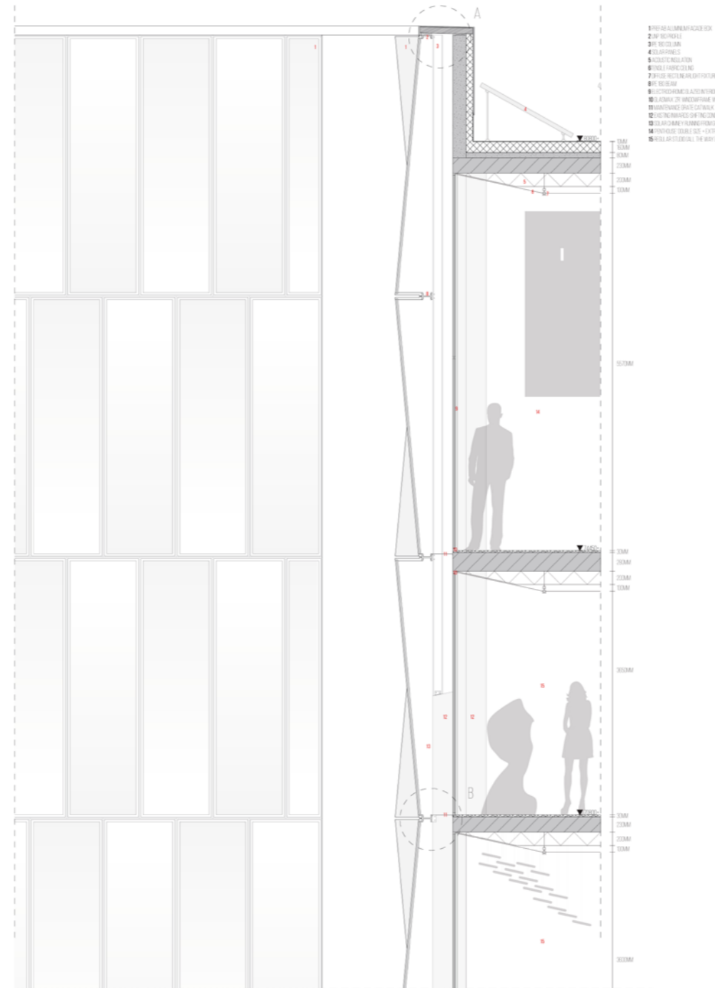
fig 2. 1:20 elevation, 1:20 section
